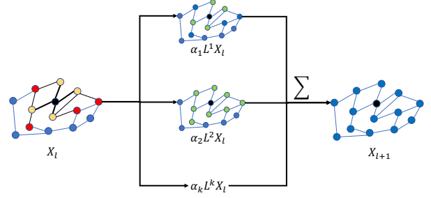
Figure 3: An example of the ChebNet graph convolution centralized at the black vertex. Left: The centralized region is marked black. The one-hop neighbors are marked yellow, while the two-hop neighbors are marked red. Middle: with the increase of degree of the graph Laplacian, the reception field grows (marks green). Right: The output of this layer is a sum among graph transformations with degree value from 1 to K .
