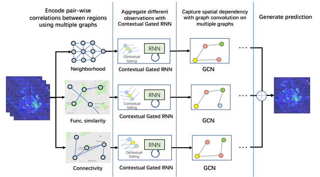
Figure 2: System architecture of the proposed spatiotemporal multi-graph convolution network (ST-MGCN). We encode different aspects of relationships among regions, including neighborhood, functional similarity and transportation connectivity, using multiple graphs. First, the proposed contextual gated recurrent neural network (CGRNN) is used to aggregate observations in different times considering the global contextual information. After that, multi-graph convolution is used to model the non-Euclidean correlations among regions.
